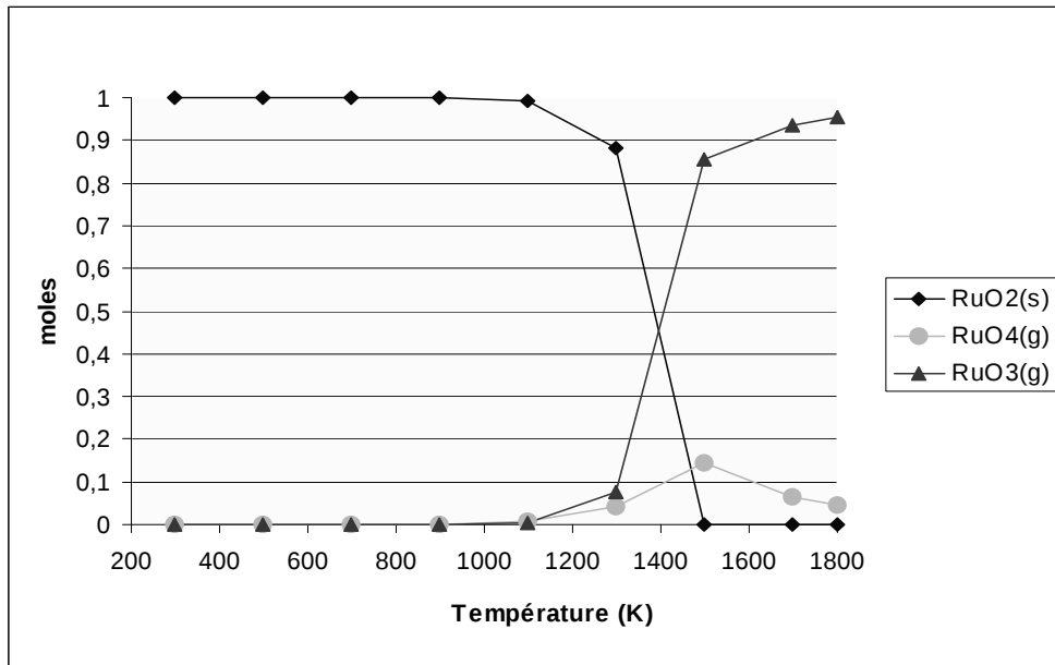
Figure 3: Thermodynamic stability of RuO 4 (g), RuO 3 (g) and RuO 2 (s) as a function of temperature for respectively 1 mole of Ru, 100 moles of H 2 O, and 200 moles of O 2 (15% molar).
