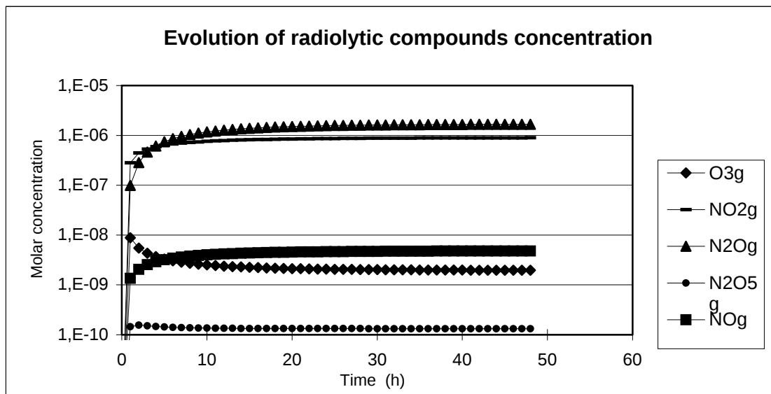
Figure 4: Air radiolysis compounds concentration profiles as a function of time (DR=10kGy.h -1 , at 373 K, steam mass fraction = 30%).
