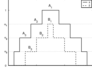
Figure 1: Comonotonic cloud
