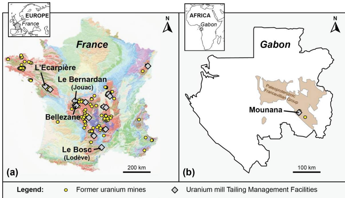
660 Figure 1: a) Geological map of France (1/1000000 series, © BRGM) and b) modified 661 geological map of Gabon (only indicating the Paleoproterozoic Francevillian Group that host 662 the U deposits; Bankole et al., 2020) showing the localization of the former uranium mines 663 and the U mill Tailing Management Facilities (France: Programme MIMAUSA database; 664 Gabon: Ossa et al., 2021). The names of the Tailing Management Facilities are reported for 665 sites where U mill tailing samples were analysed in this study.
