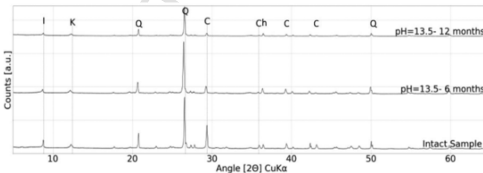
Fig. 9. X-ray diffraction profiles of three Opalinus Clay samples derivate from sample 6 from the lower sandy facies of Mont Terri site immersed in an alkaline solution with a pH = 13.5 for 6 months and 12 months respectively- I: Illite, K: Kaolinite, Ch: Chlorite, Q: Quartz, C: Calcite.
