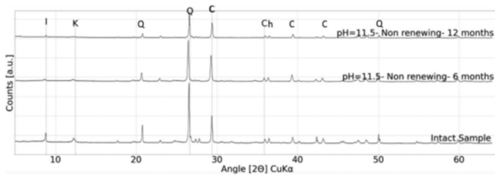
Fig. 10. X-ray diffraction profiles of three Opalinus Clay samples derivate from sample 6 from the lower sandy facies of Mont Terri site immersed in an alkaline solution initially presenting a pH = 11.5 for 6 months and 12 months respectively- I: Illite, K: Kaolinite, Ch: Chlorite, Q: Quartz, C: Calcite.
