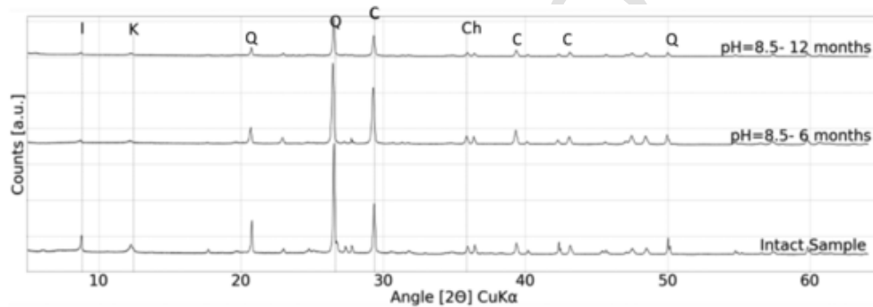
Fig. 11. X-ray diffraction profiles of three Opalinus Clay samples derivate from sample 6 from the lower sandy facies of Mont Terri site immersed in an alkaline solution with a pH = 8.5 for 6 months and 12 months respectively- I: Illite, K: Kaolinite, Ch: Chlorite, Q: Quartz, C: Calcite.
