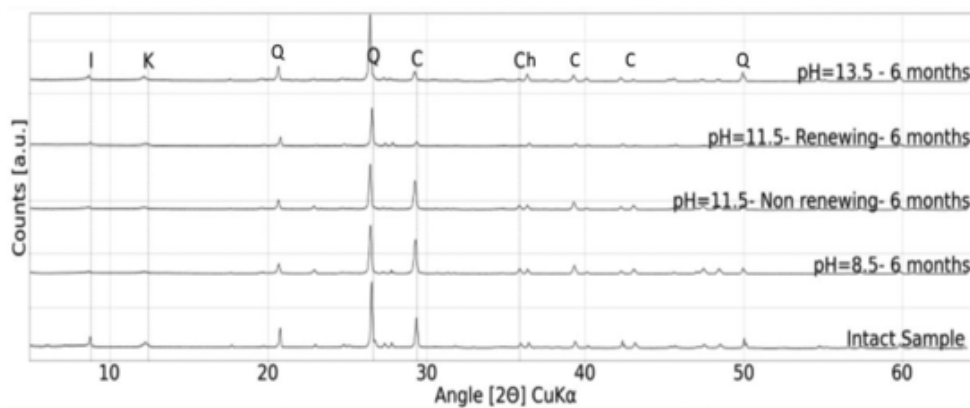
Fig. 7. X-ray diffraction profiles of four Opalinus Clay samples derivate from sample 6 from the lower sandy facies of Mont Terri site immersed in four alkaline solutions for 6 months- I: Illite, K: Kaolinite, Ch: Chlorite, Q: Quartz, C: Calcite.
