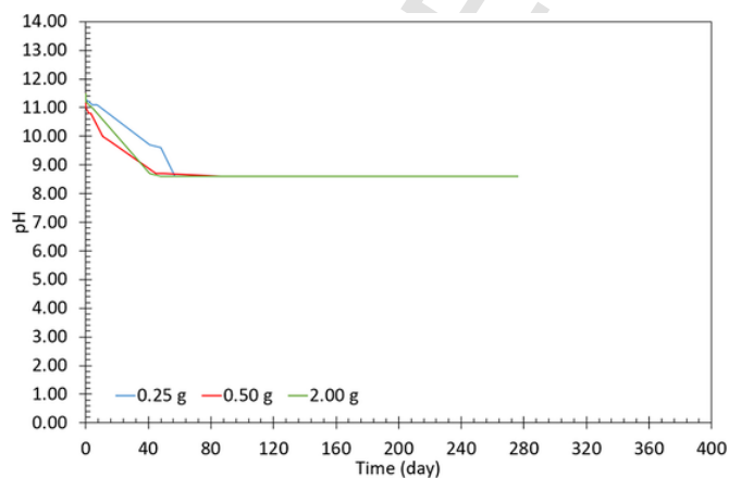
Fig. 13. pH monitoring over time for the solutions with an initial pH = 11.5 and 0.25 g (bleu curve), 0.5 g (red curve) and 2 g (green curve) of CaCO 3 .
