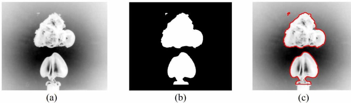
Figure 3- Image processing; (a): Sobel filter, (b): Binarization, (c): Detection of contours
