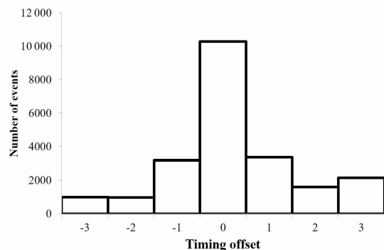
Figure 7. Histogram of the timing offset between observed and simulated peaks for the year 2021.
