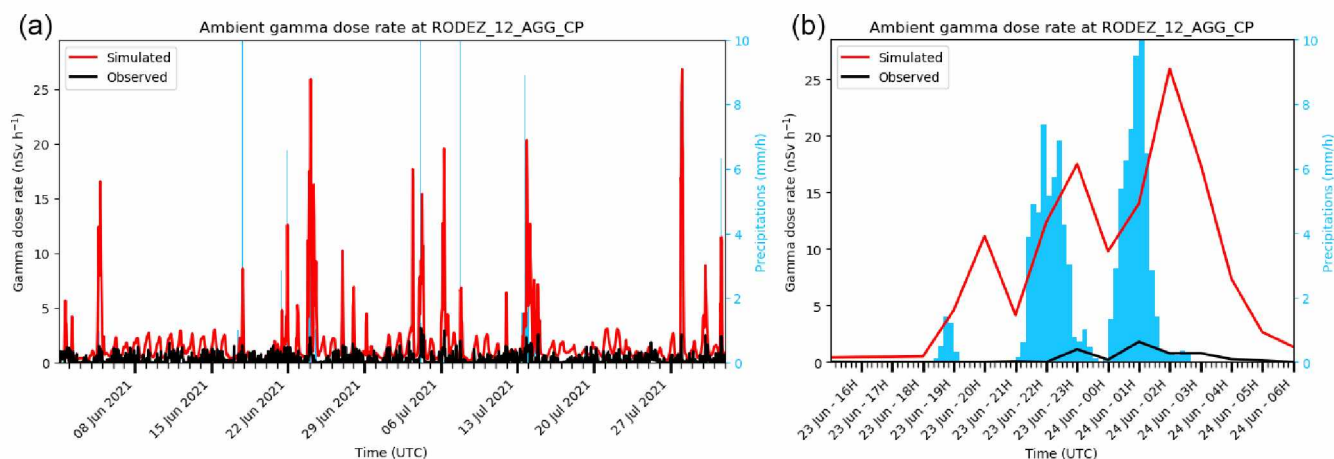
Figure 11. Observed and simulated ambient gamma dose rates at the Rodez station. (a) In June and July 2021. (b) The 24 June 2021.
