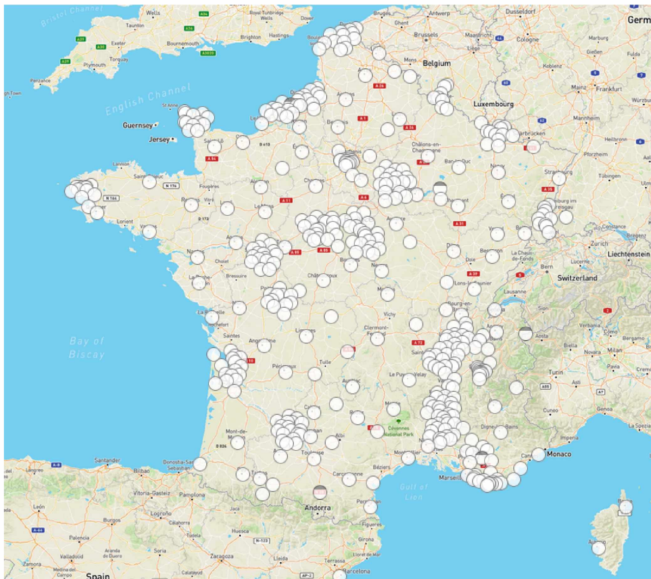
Figure 4. Téléry ambient gamma dose rate network, © Open StreetMap contributors. Distributed under the Open Data Commons Open Database License (ODbL) v1.0.
