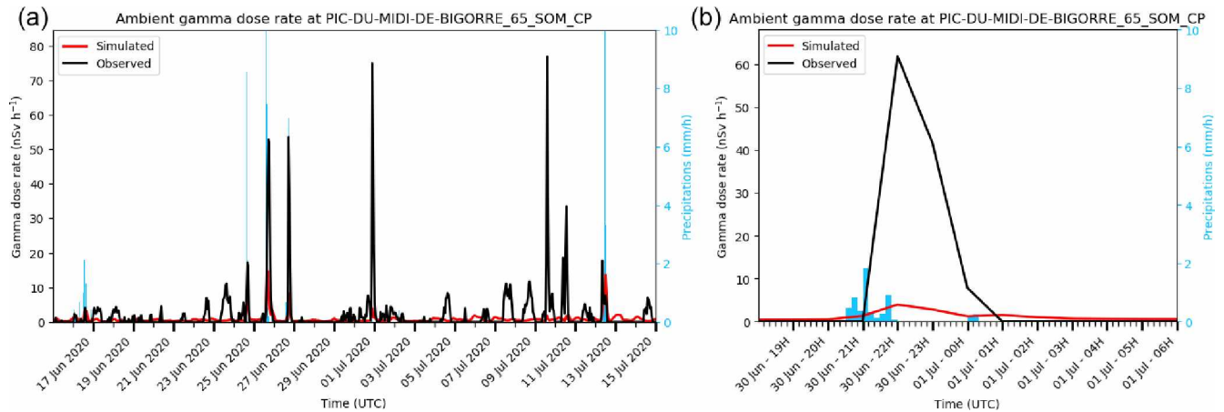
Figure 8. Observed and simulated ambient gamma dose rate at the Pic-du-Midi-de-Bigorre station. (a) In June and July 2020. (b) The 30 June 2020.
