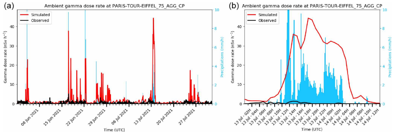
Figure 9. Observed and simulated ambient gamma dose rates at the Paris Tour Eiffel station. (a) In June and July 2021. (b) The 13 July 2021.
