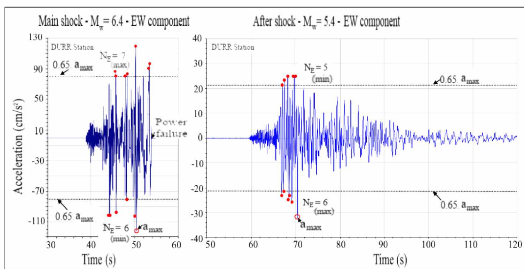
Figure 7 : Number of equivalent uniform stress cycles ( N_E ) for the main shock M_w 6.4 (left) and for an aftershock M_w 5.4 (right) recorded the same day to the Durrës station – Component EW –
