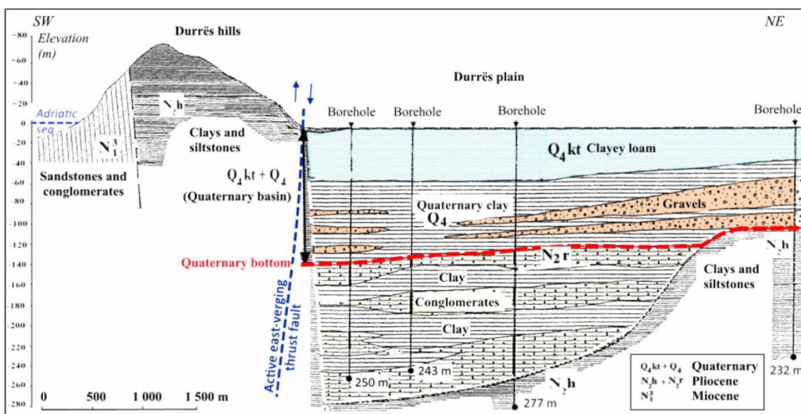
Figure 2 : Interpreted geological cross-section SW-NE of the Durrës sedimentary basin Vertical scale strongly exaggerated (Extracted and modified from UNEP report, 2001; approximate location on the Figure 1).
