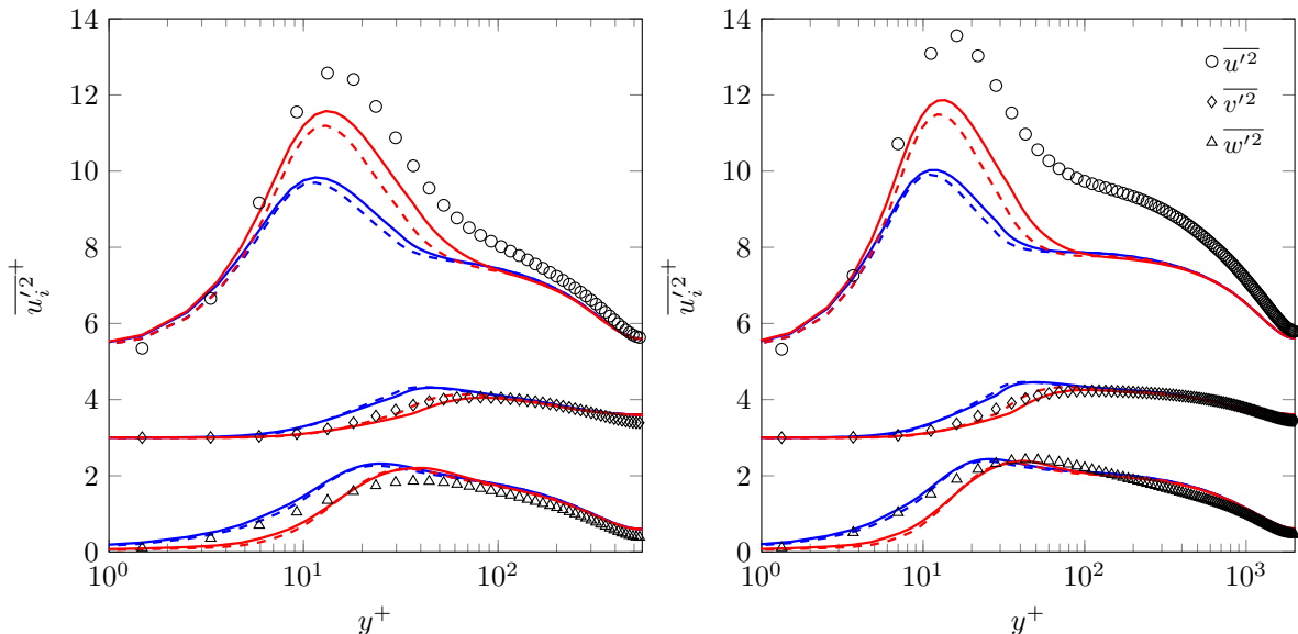
Figure 8: Turbulent channel flow. Comparison of model predictions with DNS data for the normal stresses at Re_\tau = 550 (left) and Re_\tau = 2000 (right). Legend as in Fig. 6. Streamwise and normalwise components are shifted for clarity.
