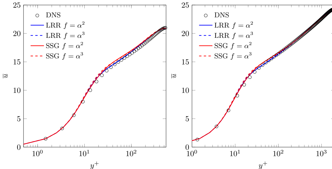
Figure 6: Turbulent channel flow. Comparison of model predictions with DNS data for the streamwise mean velocity at Re_\tau = 550 (left) and Re_\tau = 2000 (right)
