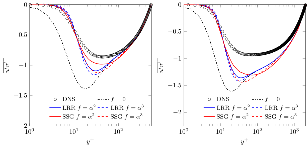
Figure 1: Turbulent channel flow. A priori test of the model for the shear component of the Reynolds stress at Re_\tau = 550 (left) and Re_\tau = 2000 (right)
