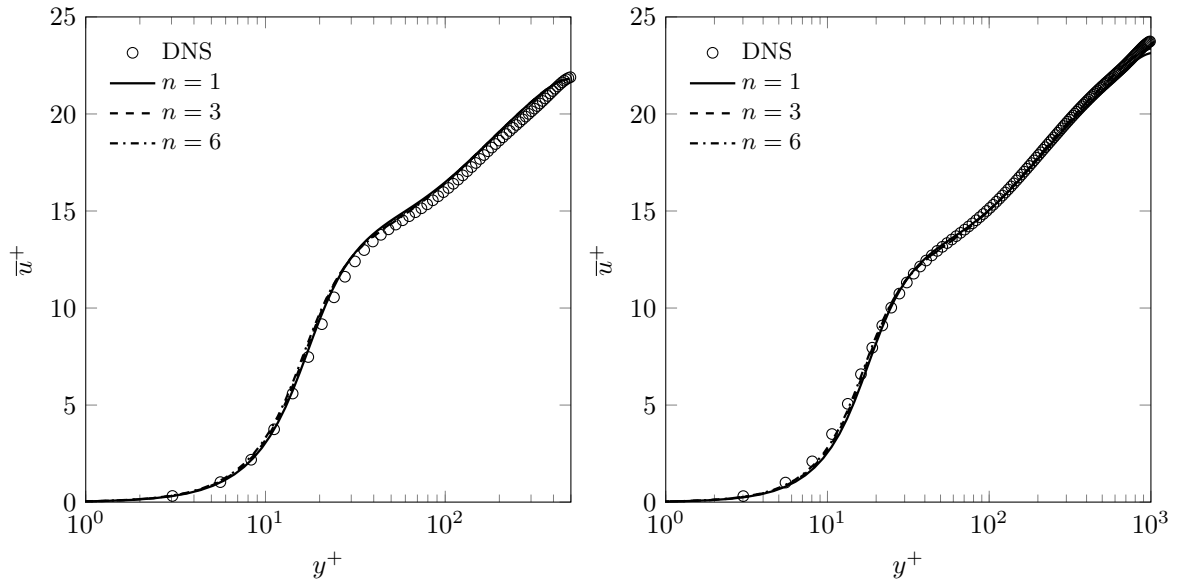
Figure 15: Square duct flow. Mean streamwise velocity along the corner bisector at Re_\tau = 500 (left) and Re_\tau = 1000 (right)
