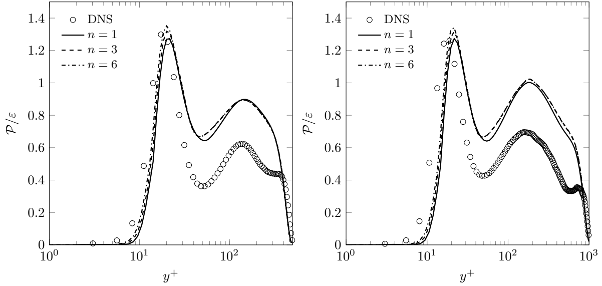
Figure 17: Square duct flow. Production-to-dissipation ratio along the corner bisector at Re_\tau = 500 (left) and Re_\tau = 1000 (right)
