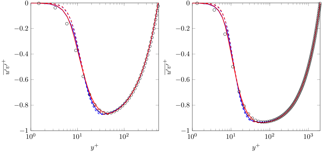
Figure 7: Turbulent channel flow. Comparison of model predictions with DNS data for the shear stress at \text{Re}_\tau = 550 (left) and \text{Re}_\tau = 2000 (right). Legend as in Fig. 6
