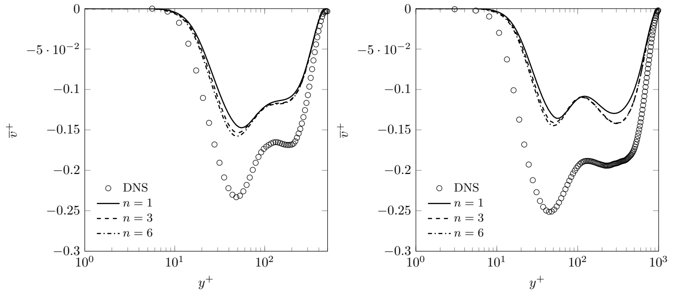
Figure 16: Square duct flow. Mean cross-wise velocity along the corner bisector at Re_\tau = 500 (left) and Re_\tau = 1000 (right)
