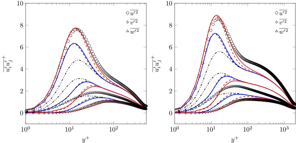
Figure 2: Turbulent channel flow. A priori test of the model for the normal component of the Reynolds stress at \text{Re}_\tau = 550 (left) and \text{Re}_\tau = 2000 (right). Legend as in Fig. 1
