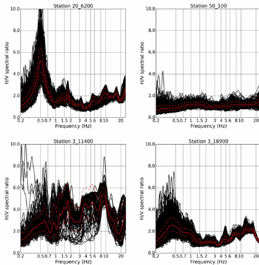
Fig. 3 – Examples of HVSR curves measured. Black lines stand for single HVSR computed on 100-s-long signals. The solid (resp. dashed) red line stands for the mean (resp. mean \pm one standard deviation) HVSR curve. The top line shows examples of interpreted HVSR curves on top of the sedimentary canyon (with a clear low frequency peak, from which f_0 is deduced, left) and on nearby rock outcrops (flat HVSR curve, right). The bottom line shows HVSR curves that were not interpreted, because of the absence of a clear peak (left) or amplitude lower than 3 (right).
