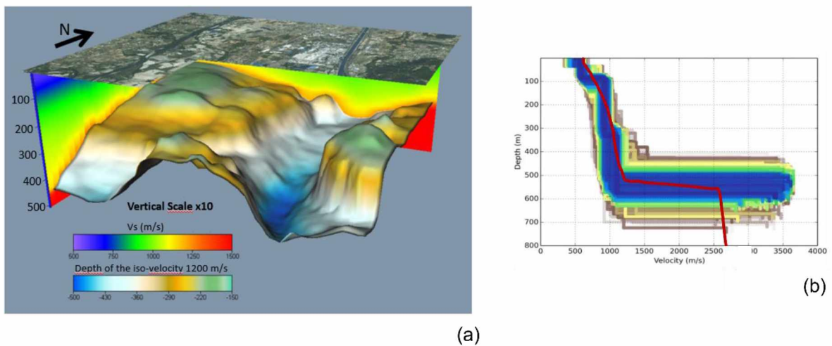
Fig. 2 - (a) Isovelocity V_s=1200 m/s surface area extracted from the Ambient Noise Surface Wave Tomography (ANSWT). (b) 1D V_s models obtained from the inversion process from Ambient Vibration Arrays (AVA) at BOLL site. Colour stands for the misfit value in the inversion procedure (from Gélis et al. 2022). The 1D velocity profile at BOLL extracted from this-study 3D V_s model is superimposed in dark red.
