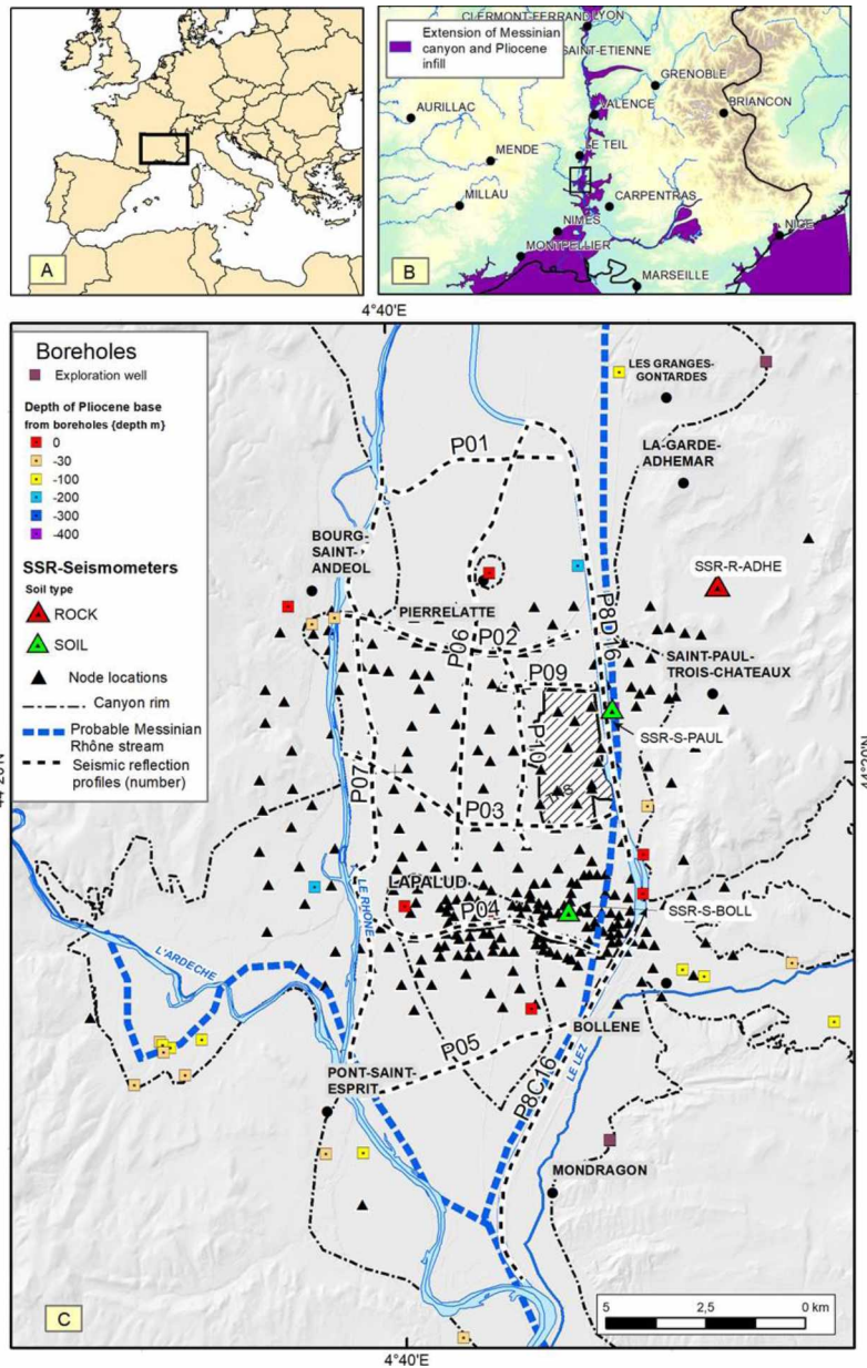
Fig. 1 – Location of datasets that have been considered in the present study: the borehole information from BSS (BRGM borehole database, coloured squares), the 11 seismic lines acquired from ENGIE company (black dashed lines) and the 400 nodes (black triangles). Note that the outline of some seismic lines may cover the triangles used to represent the 400 nodes (both experiments following the road network). For sake of clarity, we still chose to display the whole datasets on the same figure. The 3 stations (BOLL, PAUL and ADHE) deployed in previous studies are displayed as coloured triangles.
