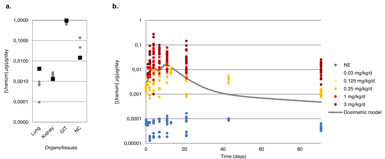
Figure 2. Uranium tissue content of mice exposed to intranasal instillation. (a) Uranium retention in lungs, kidneys, gastrointestinal tract, and nasal compartments 1 h after the first instillation to uranium of 0.25 mg/kg. Each point represents an independent animal, and the square represents the SAAM II (Simulation, analysis, and modeling software for tracer and pharmacokinetic studies) biodosimetric model, n = 4 . GIT gastro-intestinal tractus, NC nasal compartment. (b) Biodosimetric model of uranium content in the kidneys after repeated intranasal instillations (0.03–3 mg/kg/day) according to the quantity of uranium administered to mice. Each point represents an independent animal; n = 4 –12 for each time and dose.
