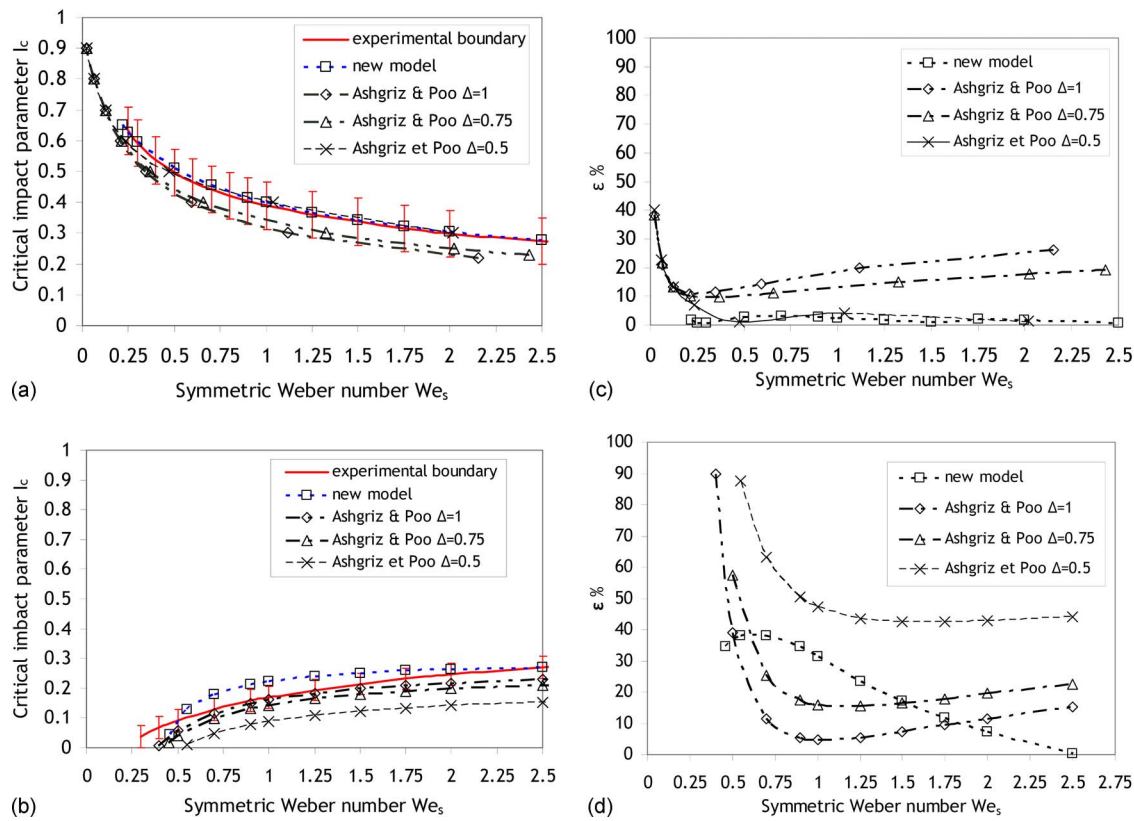
FIG. 7. (Color online) Curves for outcomes transitions: [(a) and (c)] coalescence/stretching separation and [(b) and (d)] coalescence/reflexive separation. Left: critical impact parameter, error bars represent \pm 3 standard deviations. Right: relative difference on I_c between the experimental results, and both Ashgriz and Poo (Ref. 6) expressions ( \Delta=0.5; 0.75; 1 ) and the new proposed model.
