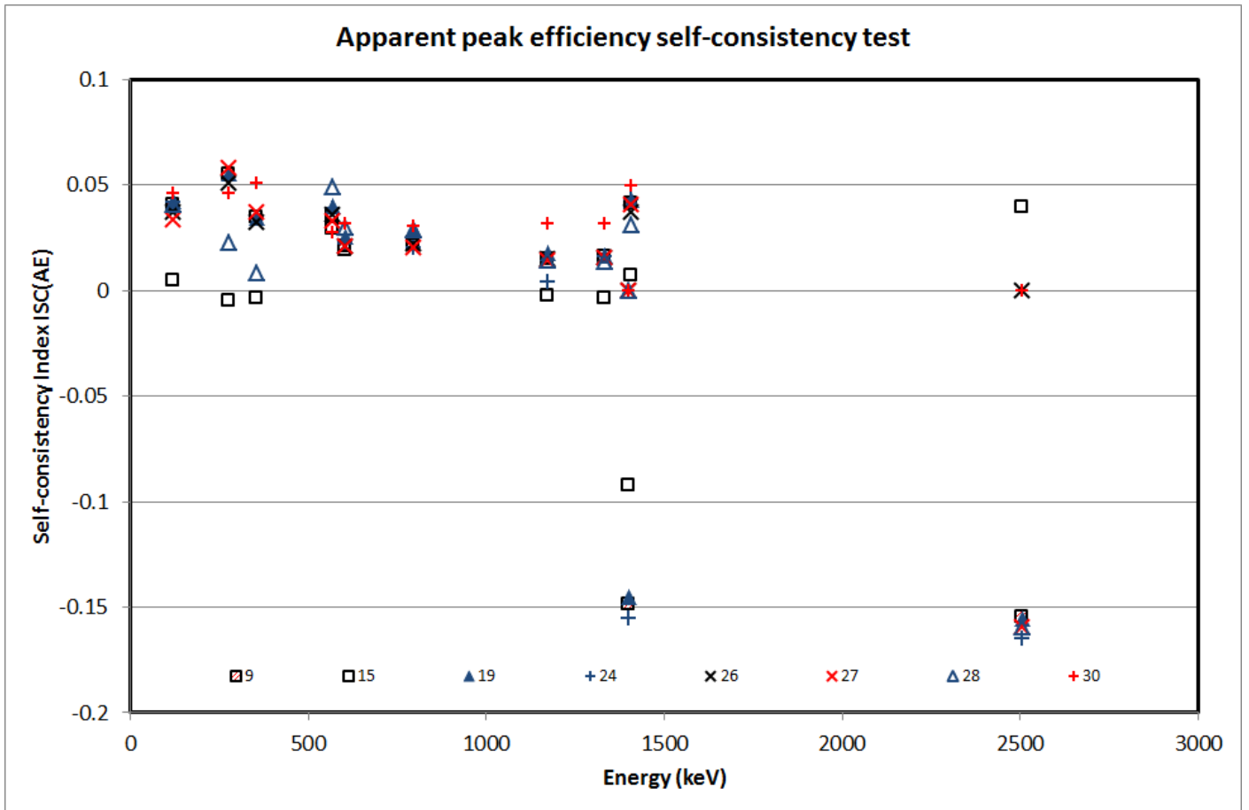
Figure 9. The self-consistency index for the apparent peak efficiency for the sets of results in which at least one absolute value of ISC(AE)>0.05. The uncertainty bars were removed for avoiding a too clumsy figure.
