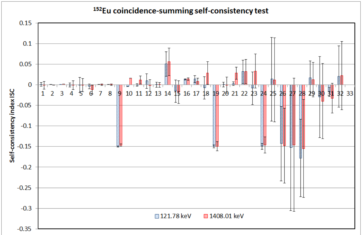
Figure 5. Self-consistency index for ^{152}\text{Eu} peaks of energy 121.78 keV and 1408.01 keV. The values of ISC(NP) are displayed in function of the code of the participants.
