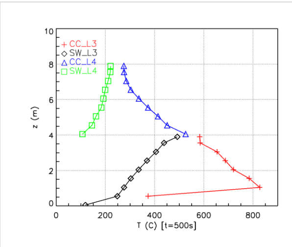
Figure 7: Vertical temperature profiles at the axis of the vent (CC) and on the SW axis in the fire room L3 ( z=[0;4] m) and in the upper room L4 ( z=[4;8] m) at t=500 s.
