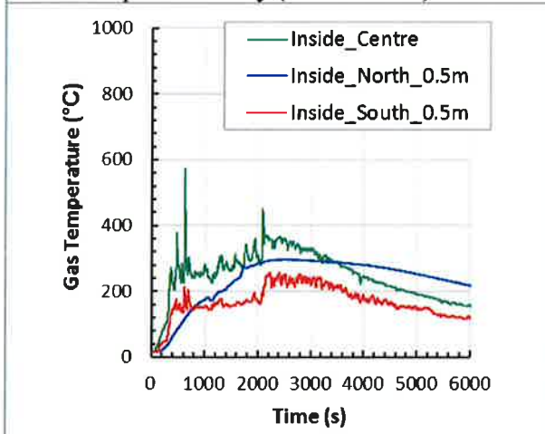
Figure 15: Gas temperature inside the lower protected tray (CORE-2 test).
