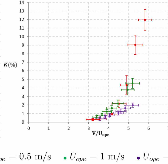
Figure 12 Evolution of the backflow factor K (%) as a function of V/U_{ope} for the case of internal transverse wall jet disturbance.
