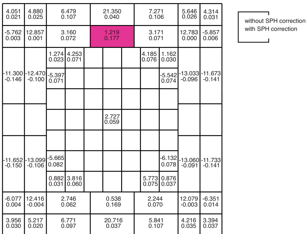
Figure 2: Percent error on the fission rates – Hafnium bars withdrawn.
