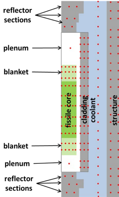
Figure 3 Axial Node Structure used in SAS-SFR code
