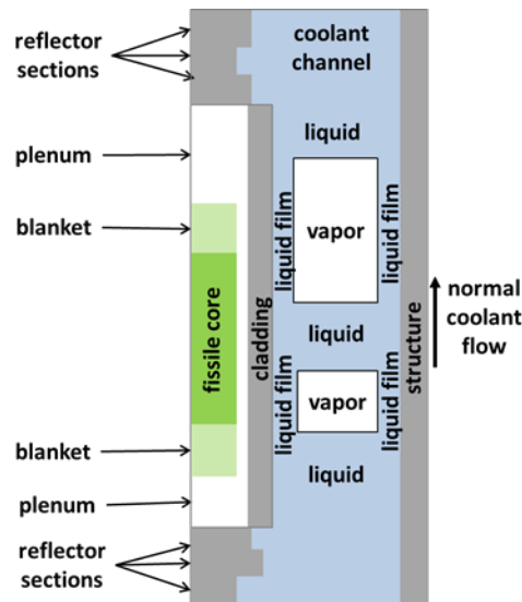
Figure 1 Representation of the multiple-bubble boiling model
