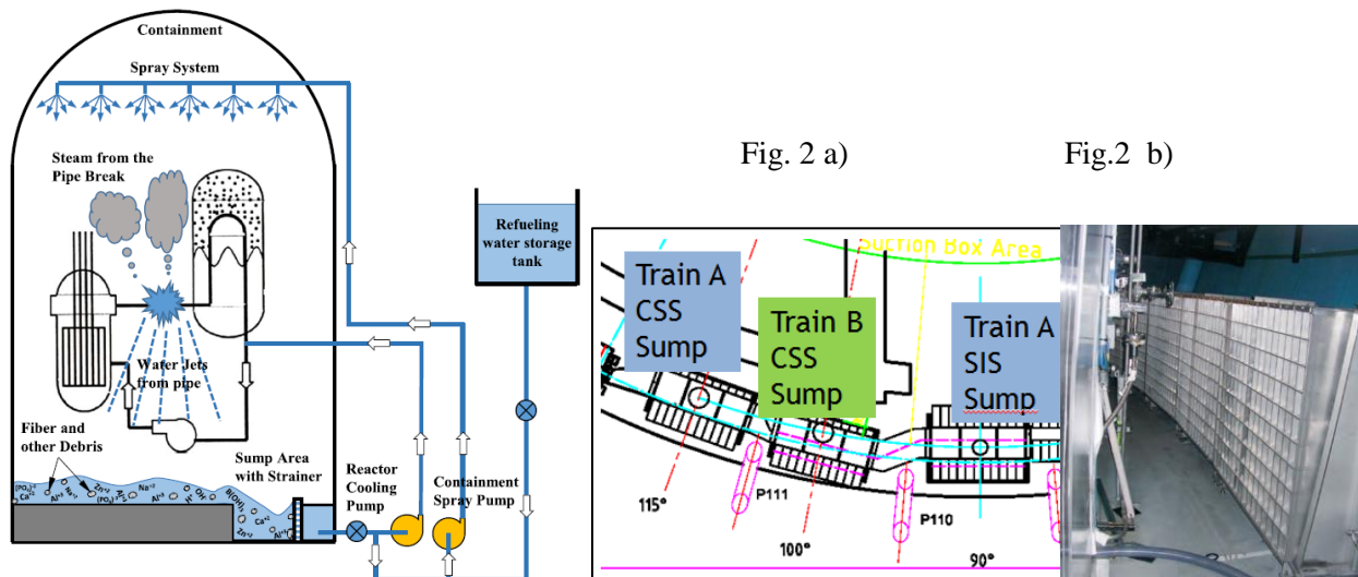
Figure 1. (left) Simplified scheme of the recirculation loop in the pressurized water reactor
