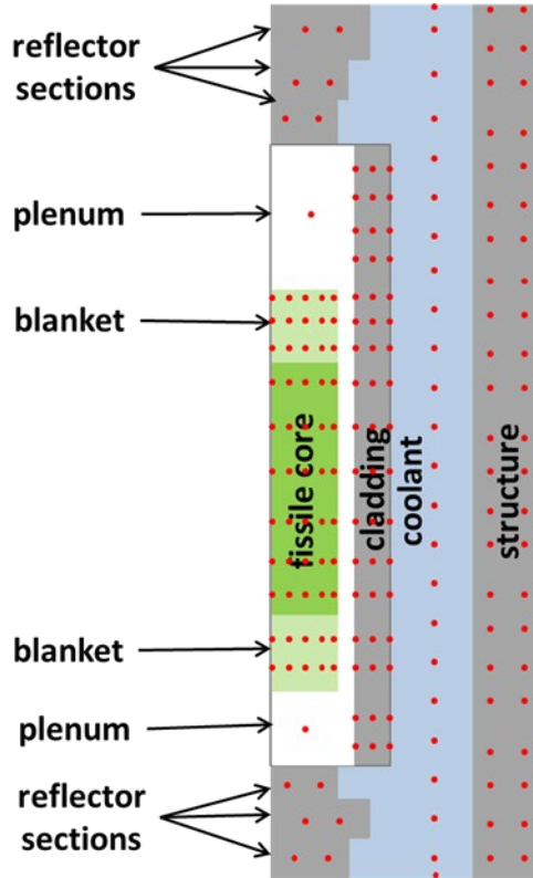
Figure 3 Axial Node Structure used in SAS-SFR code
