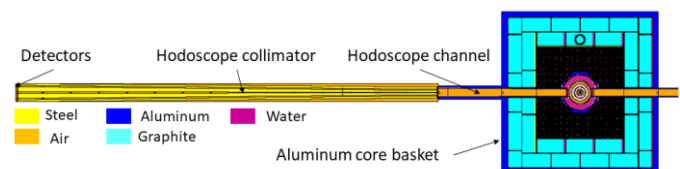
Fig. 8. MCNP6.2 radial cross section of CABRI reactor.
