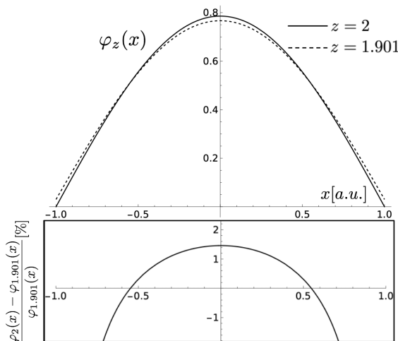
FIG. 2. Top plot: comparison between the first normalized eigenfunction of the linear diffusion equation ( z = 2 in plain line) with Dirichlet boundary conditions in -1 and 1 , and an approximation of the first normalized eigenfunction of the fractional Laplacian (as given by [40]) with z = 1.901 (dashed line). The approximation is valid far from the boundaries, i.e. within the bulk. Bottom plot: relative differences (in %) between both eigenfunctions.
