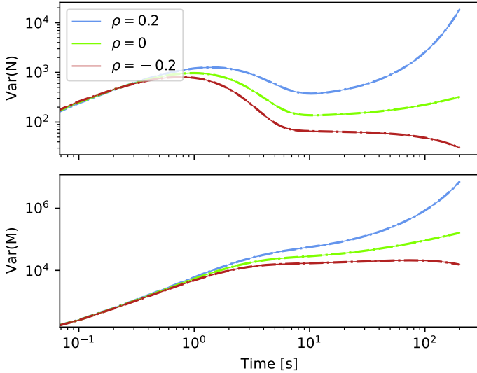
FIG. 1. Comparison of the variance of the neutron and precursor populations extracted from the solution of the stochastic process (plain lines) and from the calculation of Feynman diagrams (dotted lines), for \rho = -0.2 (red), 0 (green), 0.2 (blue). The calculations are made assuming the following set of parameters: \beta = 0.8 , \lambda_D = 0.03 , N_0 = 1000 , \bar{\nu}_n^{(2)} = 2 , \bar{\nu}_m^{(2)} = 1.2 . The two offspring distributions were supposed independent so that \frac{\bar{\nu}_m(\bar{\nu}_n - 1)}{\nu_m(\nu_n - 1)} = \frac{\beta}{1-\beta} \bar{\nu}_n^{(2)} .
