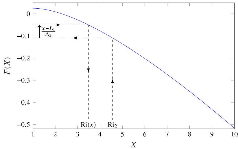
Figure 4: Graphical determination of the longitudinal evolution of the Richardson number in the subcritical region via the universal function F (the function F has been drawn for \alpha = 0.002 , C_d = 0.0065 , i.e. \kappa = 7.5 ). The blue solid line represents the function F and the dashed lines are provided to illustrate the graphical procedure.
