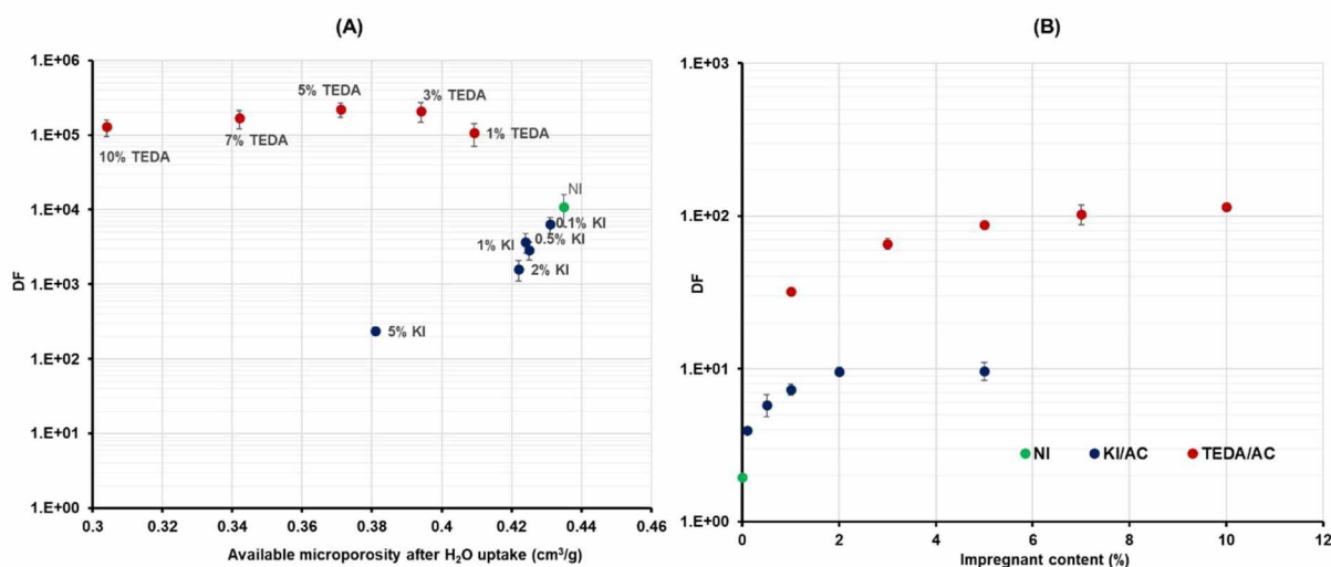
Figure 1: (A) Evolution of CH_3I retention performances for TEDA and KI impregnated AC as a function of the available microporosity calculated from N_2 porosimetry and H_2O adsorption isotherms at \{T = 20^\circ C, RH = 40\%\} . (B) Evolution of CH_3I retention performances as a function of the impregnant content at \{T = 20^\circ C, RH = 90\%\} .
