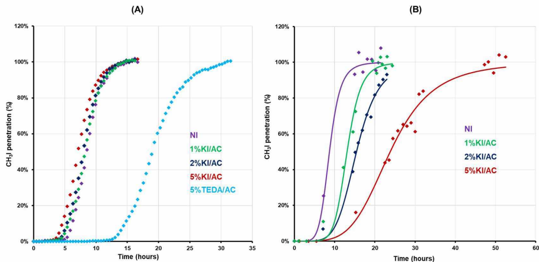
Figure 2: (A) Influence of KI and TEDA impregnations on stable \text{CH}_3\text{I} BTC at \{T = 30^\circ\text{C}, RH = 0\%\} . (B) Radioactive \text{CH}_3\text{I} BTC over KI-impregnated AC at \{T = 20^\circ\text{C}, RH = 0\%\} . The fitted curves according to an improved Thomas model are presented in lines for \gamma\text{-CH}_3\text{I} .
