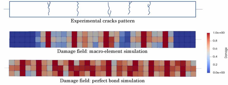
Figure 10: Concrete damage field compared to the experimental cracks pattern.
