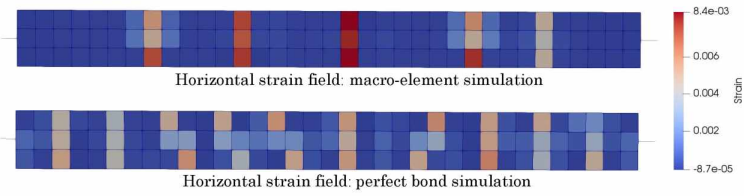
Figure 11: Horizontal concrete strain.
