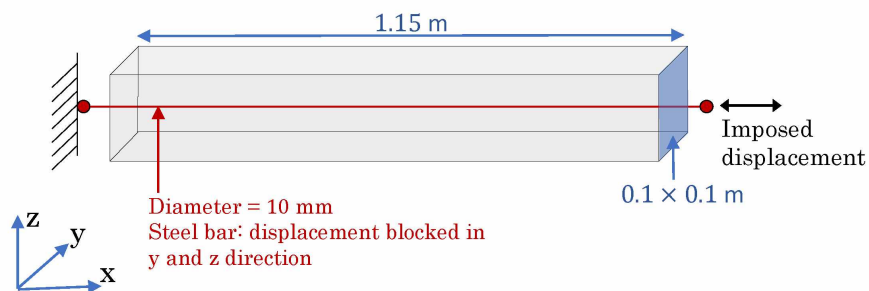
Figure 6: Presentation of the tie-rod test.
