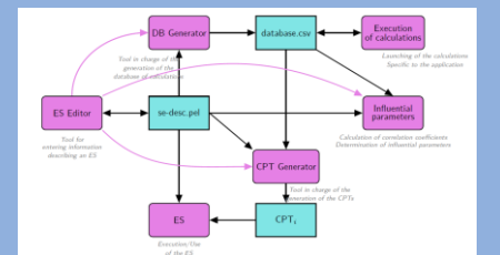
Architecture of the SE-Toolbox
