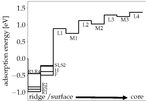
Figure 5: Energy landscape of the adsorption (formation) energies of hydrogen in \text{Be}_{318}\text{H} . The location label corresponds to ones shown in Fig. 4. Each steps correspond to stable hydrogen insertion sites.
