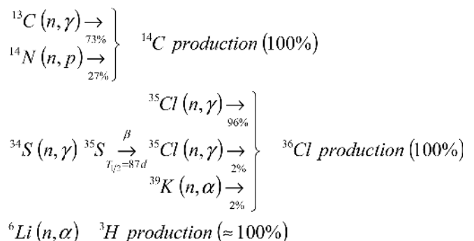
Fig. 3. Activation productions of ^{14}\text{C} , ^{36}\text{Cl} and ^3\text{H}
