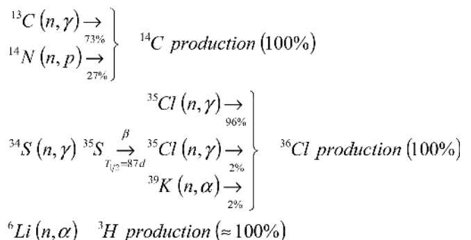
Fig. 3. Activation productions of 14 C, 36 Cl and 3 H
