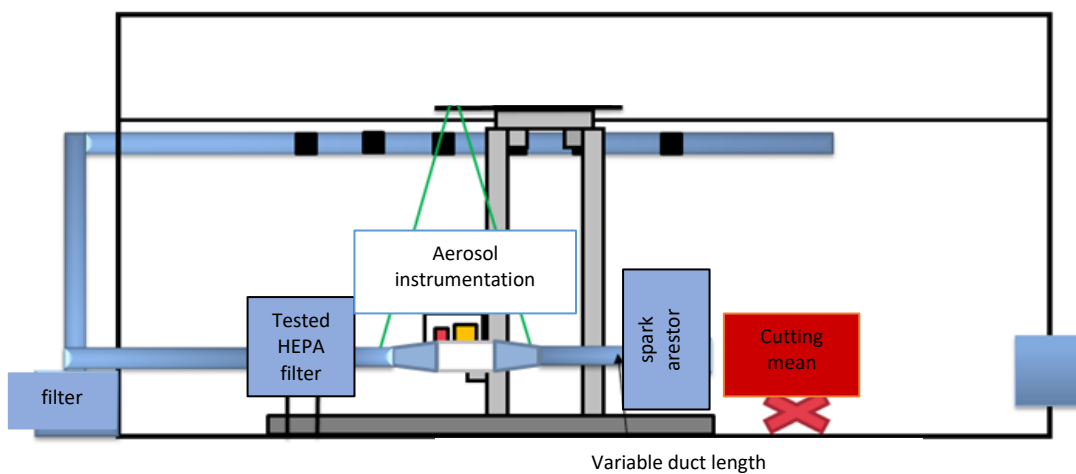
Figure 1: photo and schematic view of the test bench used in this study
