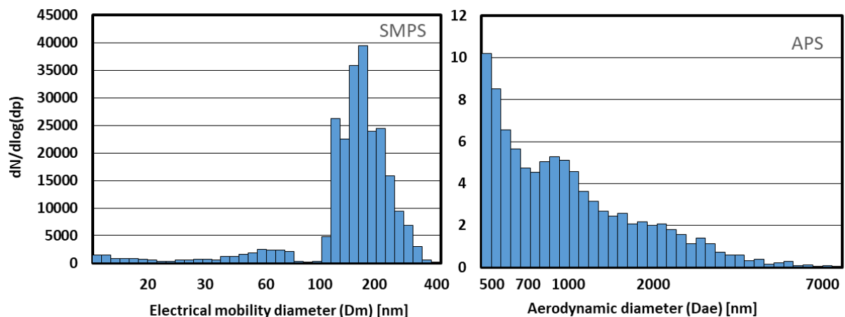
Figure 5: particle size distribution measured upstream the filter for a plasma torch cutting ((a) SMPS, (b) APS)
