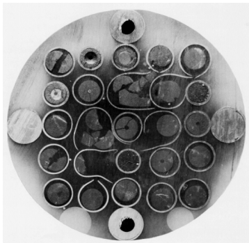
Figure 1. Bundle of deformed fuel rods Phebus LOCA experiments (1983)
