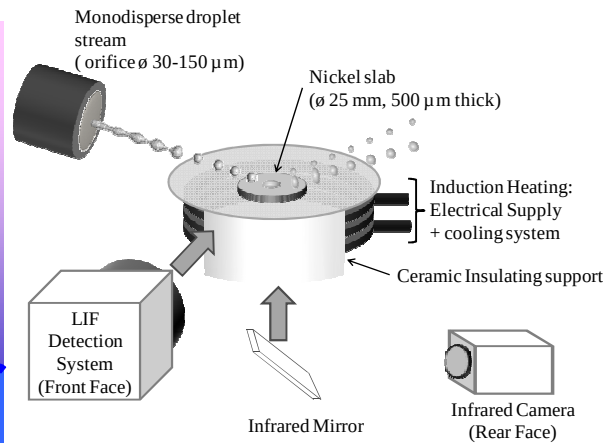
Figure. 13: Temperature measurement
