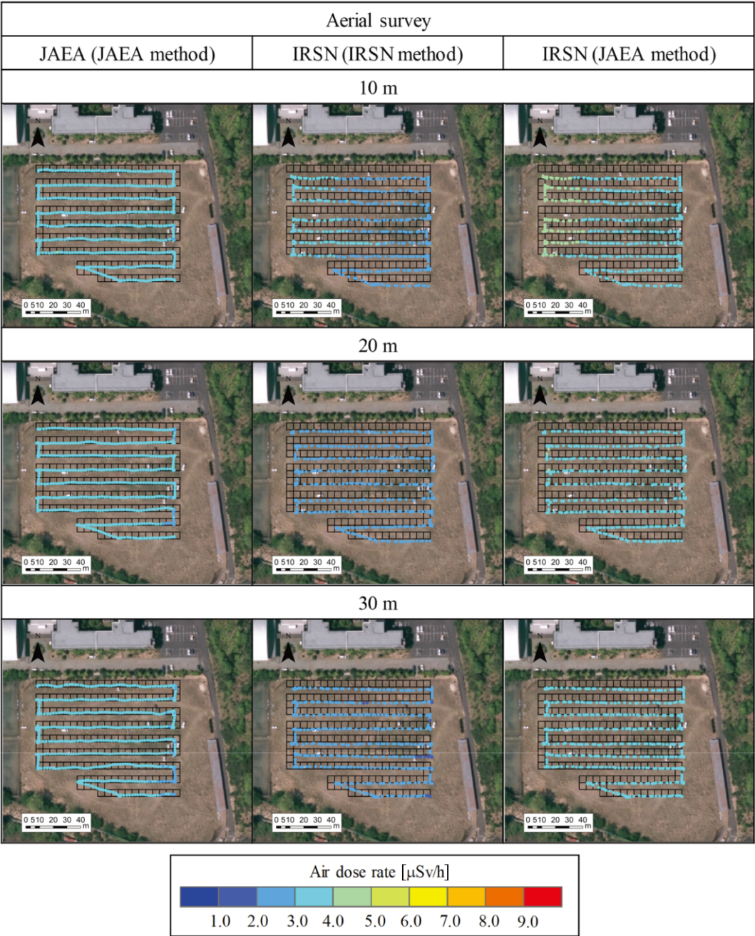
Fig. 10. Distribution of air dose rates at 1 m agl. obtained by airborne survey in site A. This map was created using ArcGIS 10.6.1.
