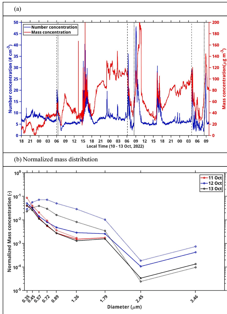
Fig. 5. Particle size distribution during the 11–13 October 2022 fog events (a) Time series of the total particle number concentration ( 0.3\text{--}20\text{ }\mu\text{m} ; \# \text{ cm}^{-3} ) from the OPC (blue line) and mass concentration ( \mu\text{g m}^{-3} ) from DataRam4 (Red line) at 2-m height, and (b) Normalized mass concentration distribution from the OPC for the three consecutive fog cases. Solid (dotted) lines indicate the average mass distribution 1 h before (during) the fog occurrence. (c) Normalized mass size distribution for all fog events.
