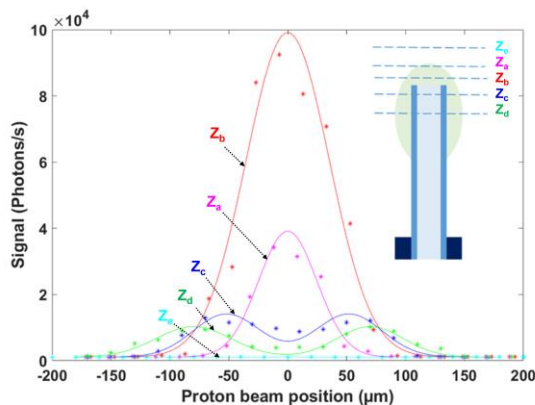
Fig. 6. Luminescence signal variations with proton beam impact position on the bulb along Y axis in different Z-planes (a) the proton beam scans nearby the bulb end, (b) beam crosses the head nearby the fiber core tip, (c) beam crosses the fiber core and cladding, (d) beam crosses fiber core and cladding far from fiber tip, (e) beam scans just above the bulb. The lines serve as visual guides.
