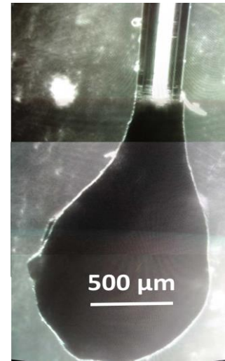
Fig. 1. Optical bright field micrograph of the ISD.
