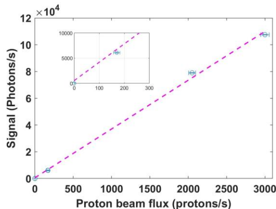
Fig. 8. Variation of photon counter signal with incident proton beam flux.
