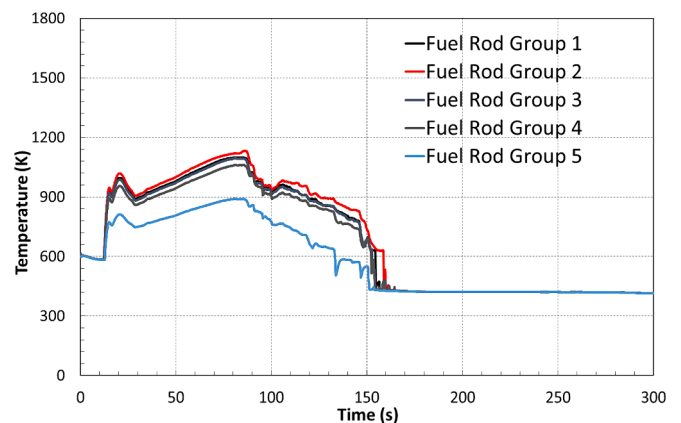
Fig. 4.8. Maximum cladding temperature (PCT) in the 5 groups of fuel rods (DBA).
