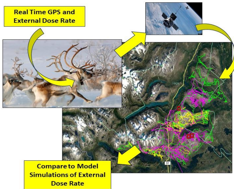
Figure 2. Depiction of GPS-coupled dosimeter on a collared reindeer (Bæk et al., 2023). The animal's physical location and external dose are sent to researchers, via satellites, at a user-defined interval. External dose rates can then be compared to model simulations.
