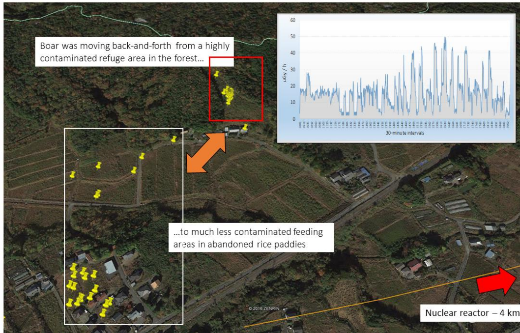
Figure 4. Variation in external dose rate observed for a wild boar living within 4- km of the damaged nuclear reactor at Fukushima. Yellow pins are the physical locations of the boar as determined by GPS data. Dose rates over time (insert) decreased when the boar went into the abandoned rice paddies, and peaked when it sought refuge in the highly contaminated forest.
