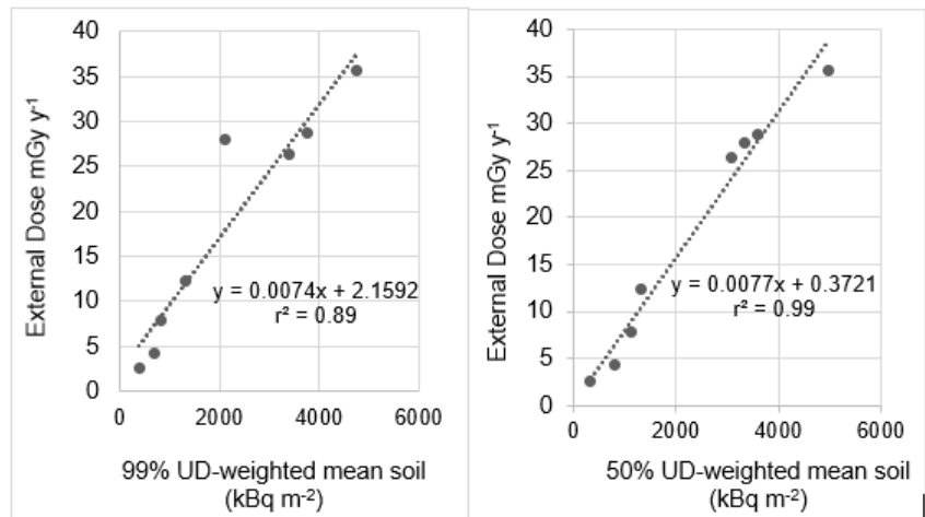
Figure 5. Correlations between weighted mean soil 137 Cs densities in wolf home ranges (99 % Utilization Distribution; left panel) and core areas (50 % Utilization Distribution; right panel) at Chernobyl with external dose rates from GPS-dosimeters worn on individual animals (Hinton et al., 2019).
