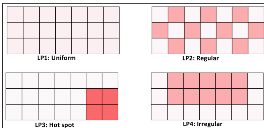
Figure 1: The 4 types of loading pattern tested in MIDI facility.
