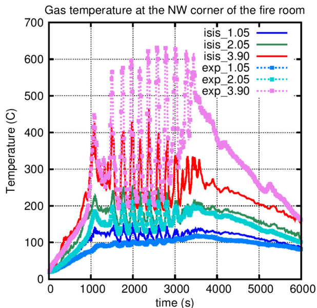
FIGURE 16 Gas temperatures at the NW corner of the fire room for the CFS-3 test [Colour figure can be viewed at wileyonlinelibrary.com ]
