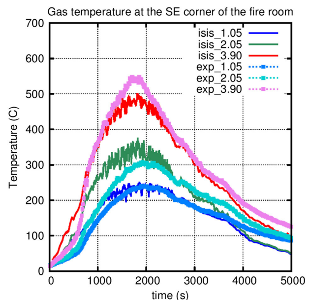
FIGURE 24 Gas temperatures at the SE corner of the fire room for the CFS-4 test [Colour figure can be viewed at wileyonlinelibrary.com]
