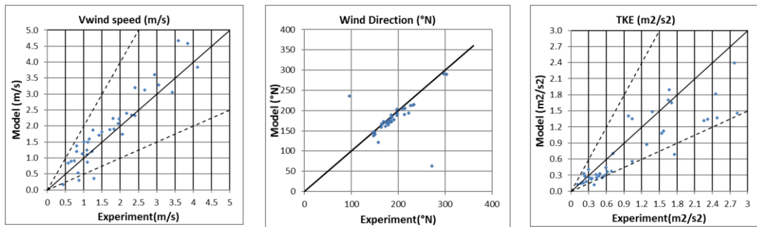
Figure 1: Scatter plots of the model/experiment comparison for wind speed, wind direction and TKE
