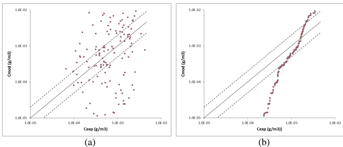
Figure 2: (a) Scatter plot and (b)Q-Q plot of predicted versus observed concentration
