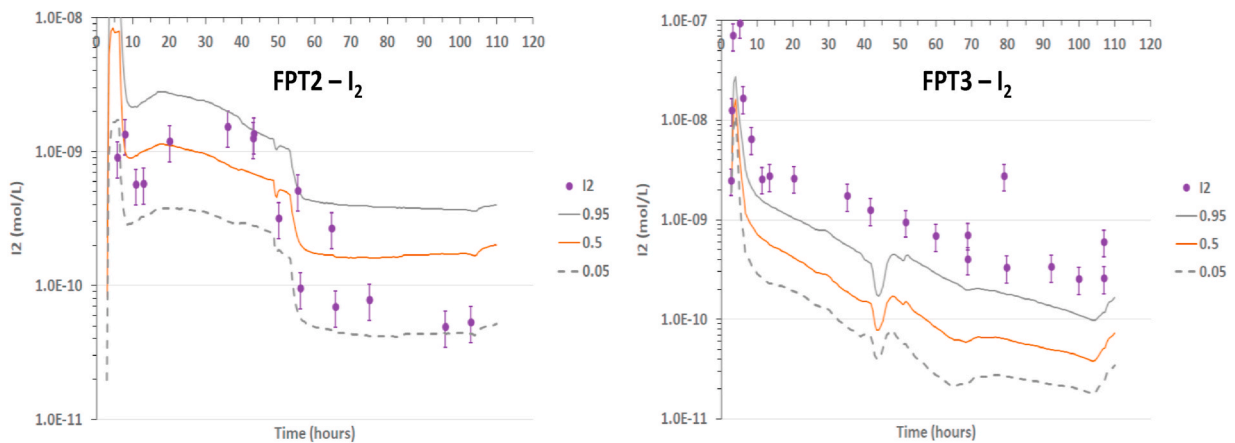
Fig. 8. Comparison data-modeling for I_2 volatility for FPT-2 (left) and FPT-3 (right) considering the 0.05/0.5/0.95 percentiles.
