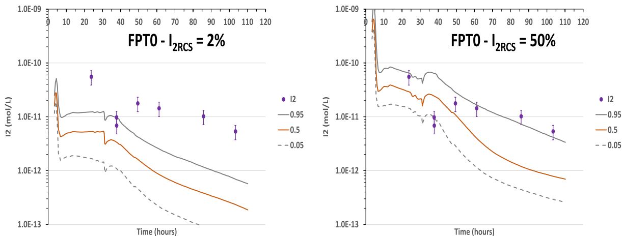
Fig. 22. Comparison data-modeling for I_2 volatility for FPT-0 considering a low \%I_{2RCS} (2%, left) and a high \%I_{2RCS} (50%, right) with the 0.05/0.5/0.95 percentiles.
