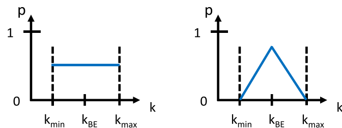
Fig. 6. Comparison of the uniform and triangle distribution functions.
