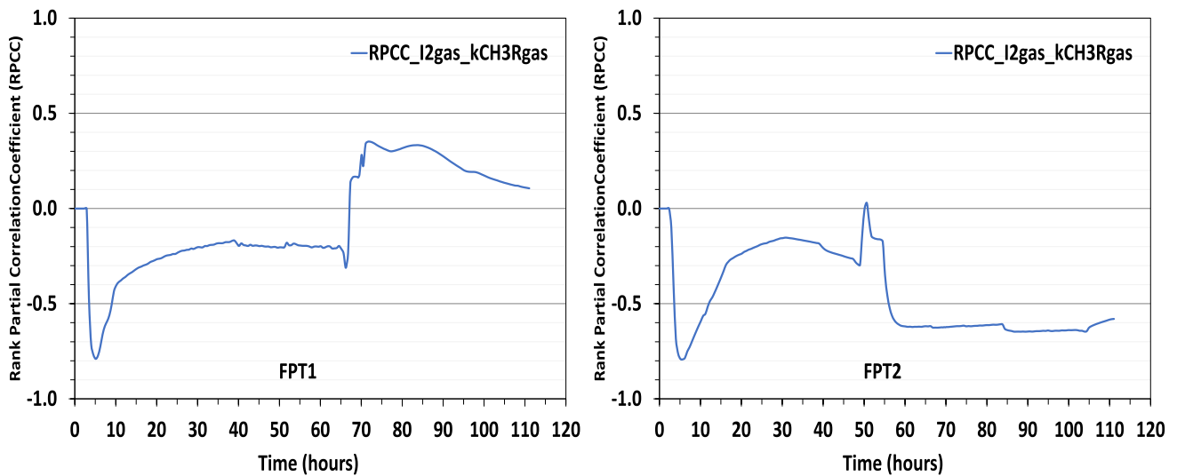
Fig. 16. Evolution of the RPCC of k_{\text{CH}_3\text{Rgas}} on \text{I}_{2\text{gas}} for FPT-1 (left) and FPT-2 (right).
