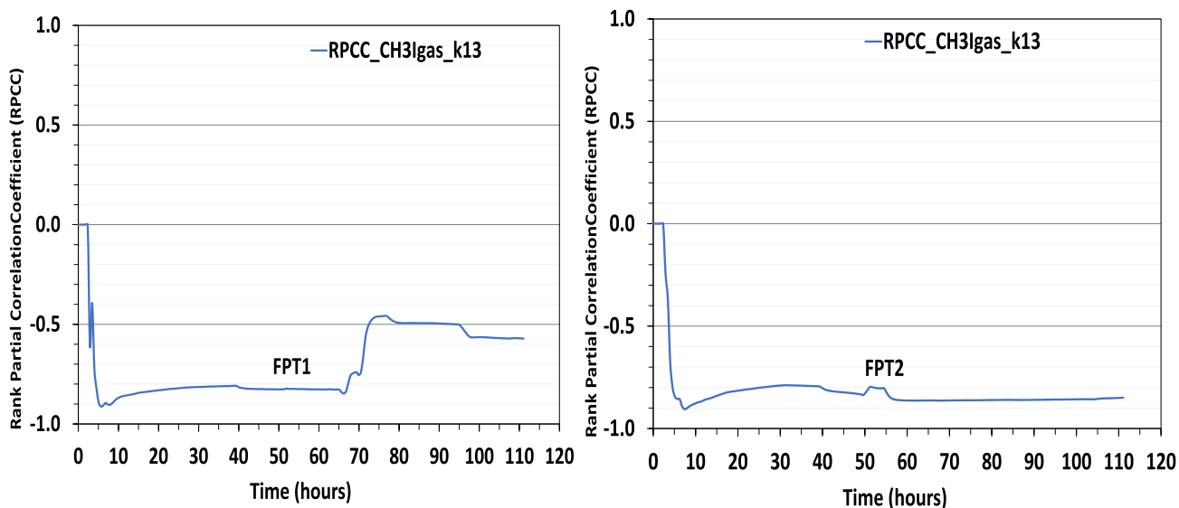
Fig. 20. Evolution of the RPCC of k_{13} on CH_3I_{gas} for FPT-1 (left) and FPT-2 (right).
