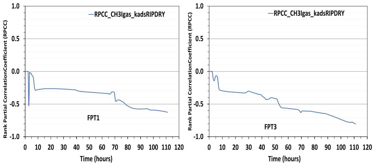
Fig. 21. Evolution of the RPCC of k_{adsRIPDRY} on CH_3I_{gas} for FPT-1 (left) and FPT-3 (right).
