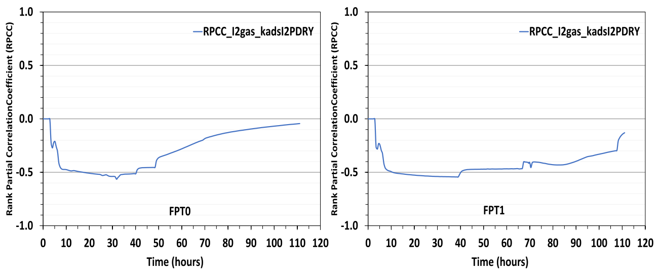
Fig. 17. Evolution of the RPCC of k_{\text{adsI}_2\text{PDRY}} on \text{I}_{2\text{gas}} for FPT-0 (left) and FPT-1 (right).
