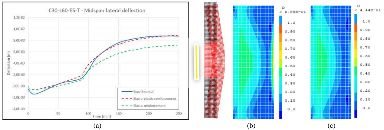
Figure 7. Comparison between experimental and computed results (a) & damage at the middle third of the column at the end of the test obtained with perfectly plastic reinforcement (b) and elastic reinforcement (c) for C30-L60-E5-T
