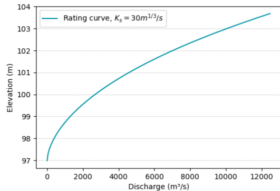
Figure 6: Stage-discharge curve
