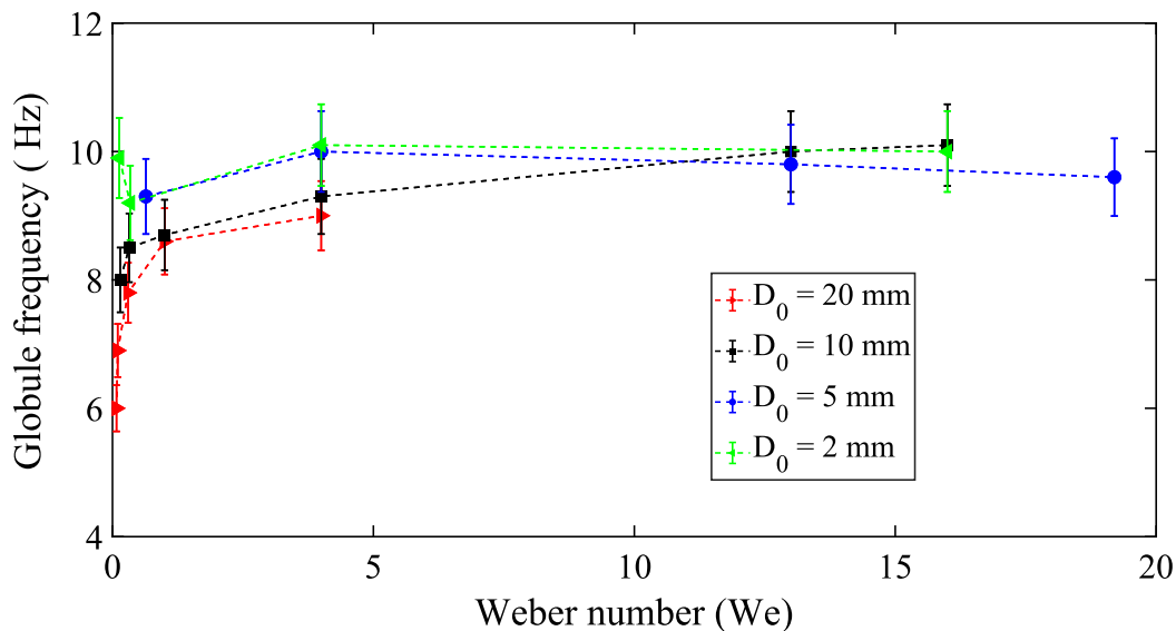
Figure III.41- Globule frequencies for different nozzles.
