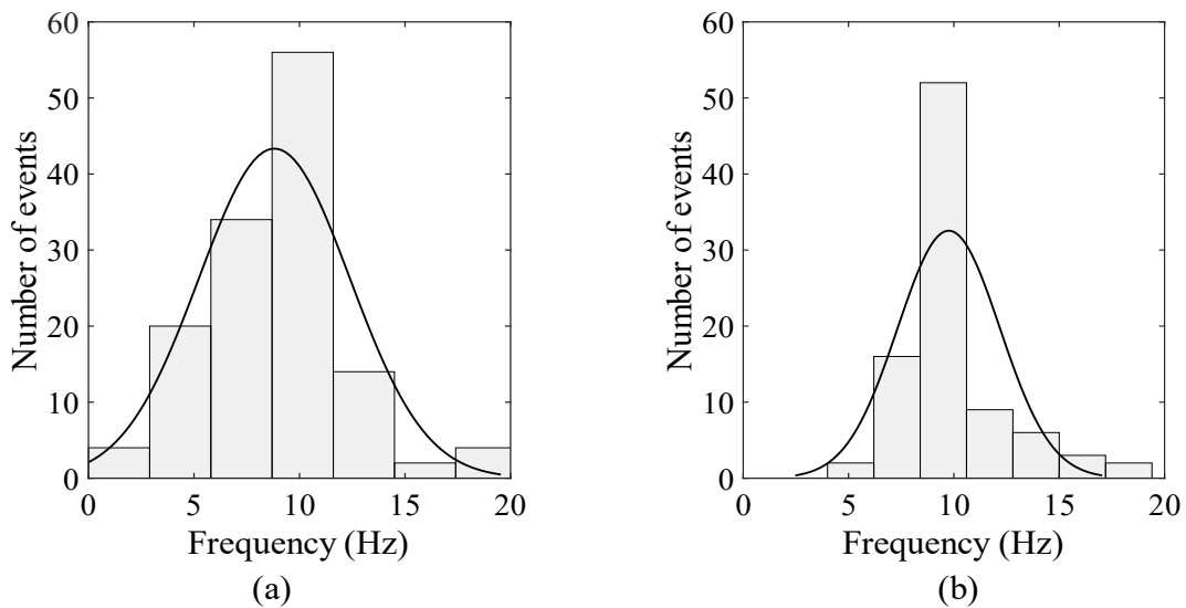
Figure III.10- Histograms of departure frequency f_b ; (a): Q_{inj} = 6 \text{ L/min} ( We = 0.16 ), (b): Q_{inj} = 36 \text{ L/min} ( We = 5.7 ).
