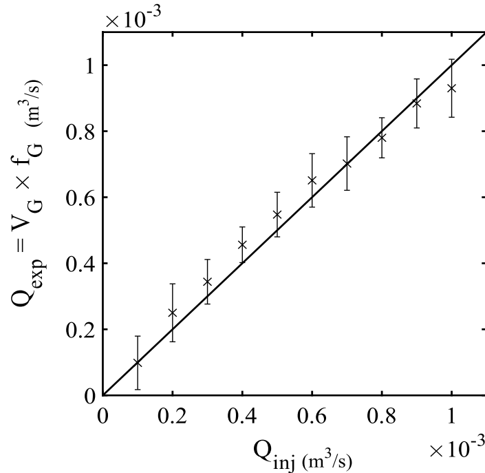
Figure III.24- Validation of the experimental flowrate with the real injected flowrate Q_{\text{inj}} .
