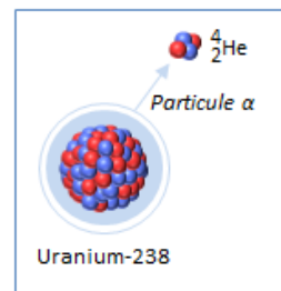
Figure 3 : Particule alpha
